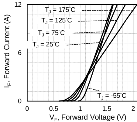
Fig.1 Forward Characteristics
