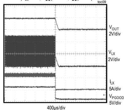
SHUTDOWN WAVEFORMS ( V_{IN} = 5\text{V} , V_{OUT} = 1.8\text{V} , I_{OUT} = 6\text{A} )
