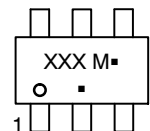
TSOP-6 CASE 318G STYLE 1
