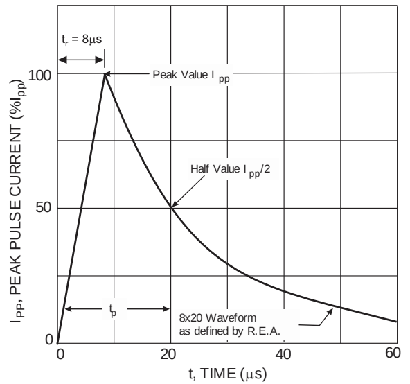
Figure 8 Pulse Waveform
