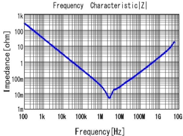
■ GRM21BB31E106KA73 |Z| DC0V, 20degC
