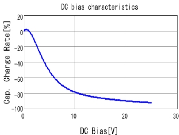
■ GRM21BB31E106KA73 C-DC bias capchange, 20.0degC, AC1.
