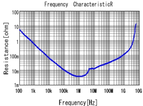
■ GRM21BB31E106KA73 R DC0V, 20degC
