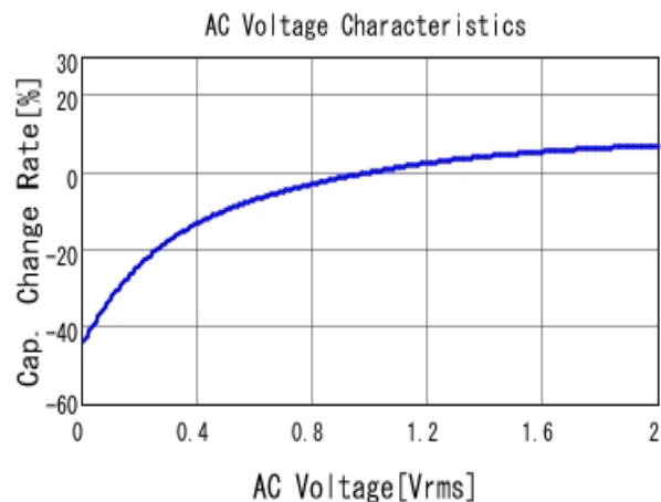
■ GRM21BB31E106KA73 C-AC Voltage capchange, DC0V, 20.0d
