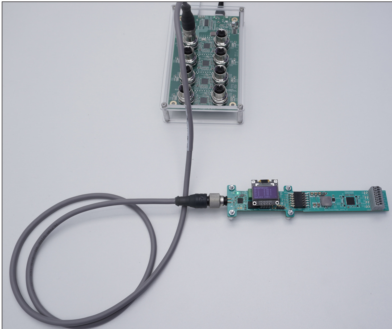
Figure 3. MAXREFDES145# + MAXREFDES281# + MAX22007PMB#.
