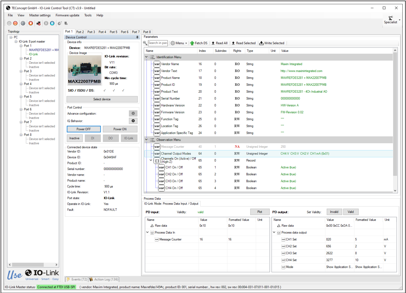
Figure 4. The TEconcept IO-Link control tool.
