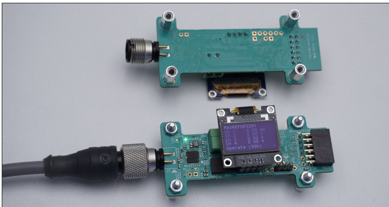
Figure 1. MAXREFDES281# IO-Link to peripheral module device.
