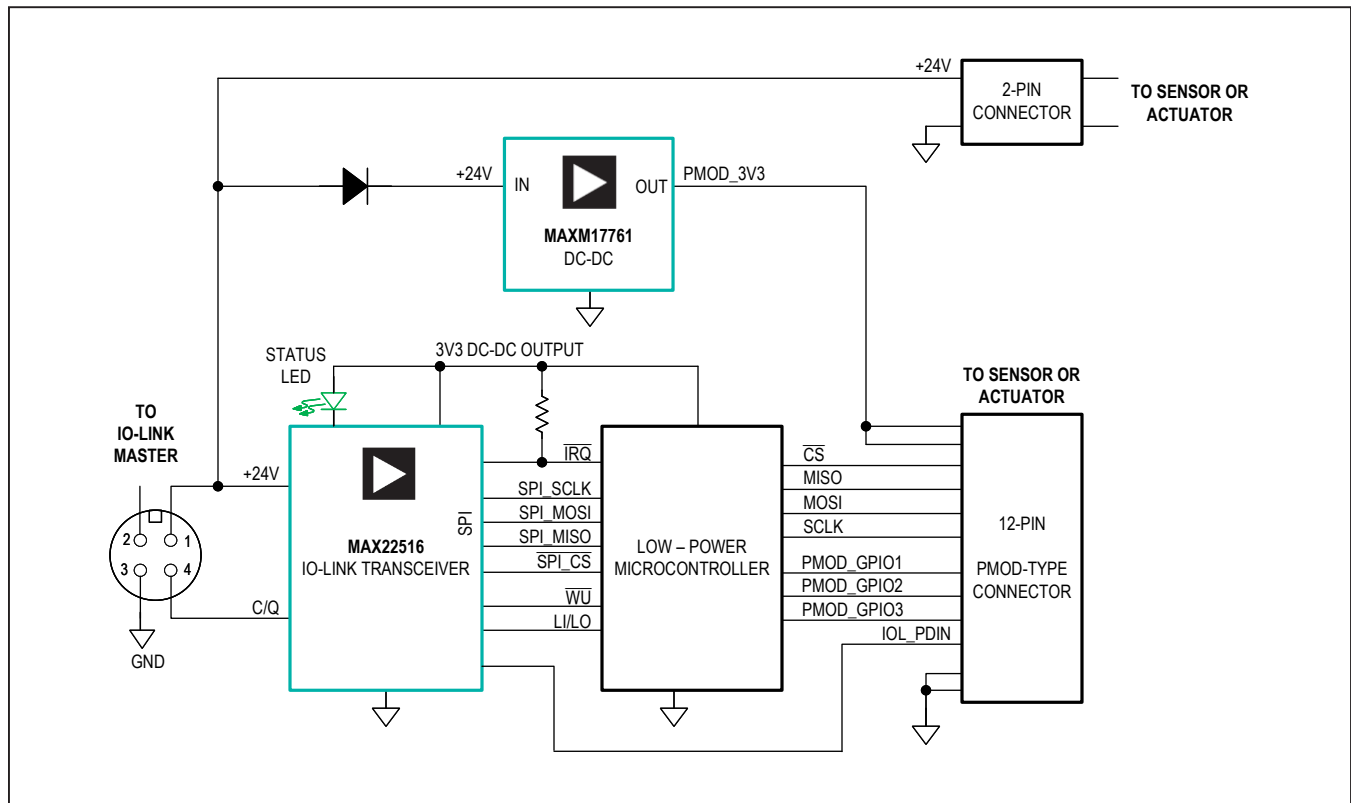
Figure 2. MAXREFDES281# system block diagram.
