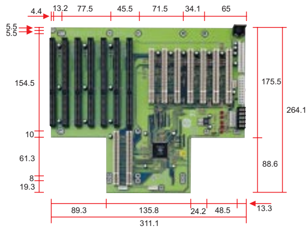
BP-214SG-P7 7 x PCI, 5 x ISA, 2 x PICMG Slot
