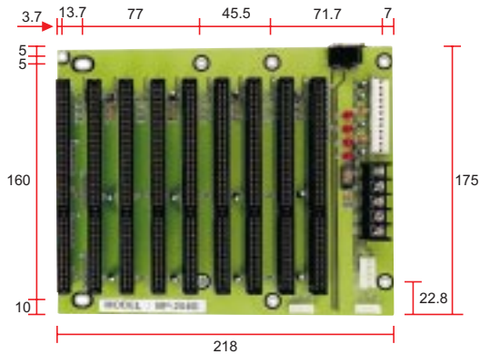
BP-208SI 8-slot ISA Backplane
