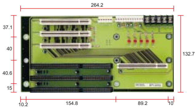
BP-206SG-P3 3 x PCI, 2 x ISA, 1 x PICMG Slot
