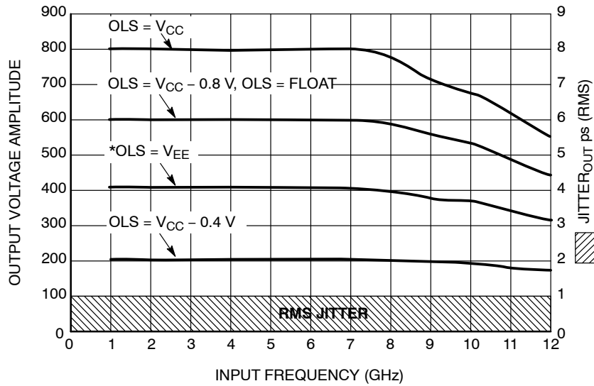
Figure 4. Output Voltage Amplitude (V OUTPP ) / RMS Jitter vs. Input Frequency (f in ) for DFF Mode (V CC - V EE = 3.3 V @ 25°C; Repetitive 1010 Input Data Pattern)
