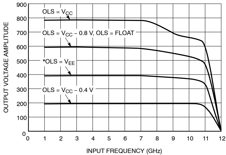
Figure 5. Output Voltage Amplitude (V OUTPP ) / RMS Jitter vs. Input Frequency (f in ) for DIV/2 Mode (V CC - V EE = 3.3 V @ 25°C)
