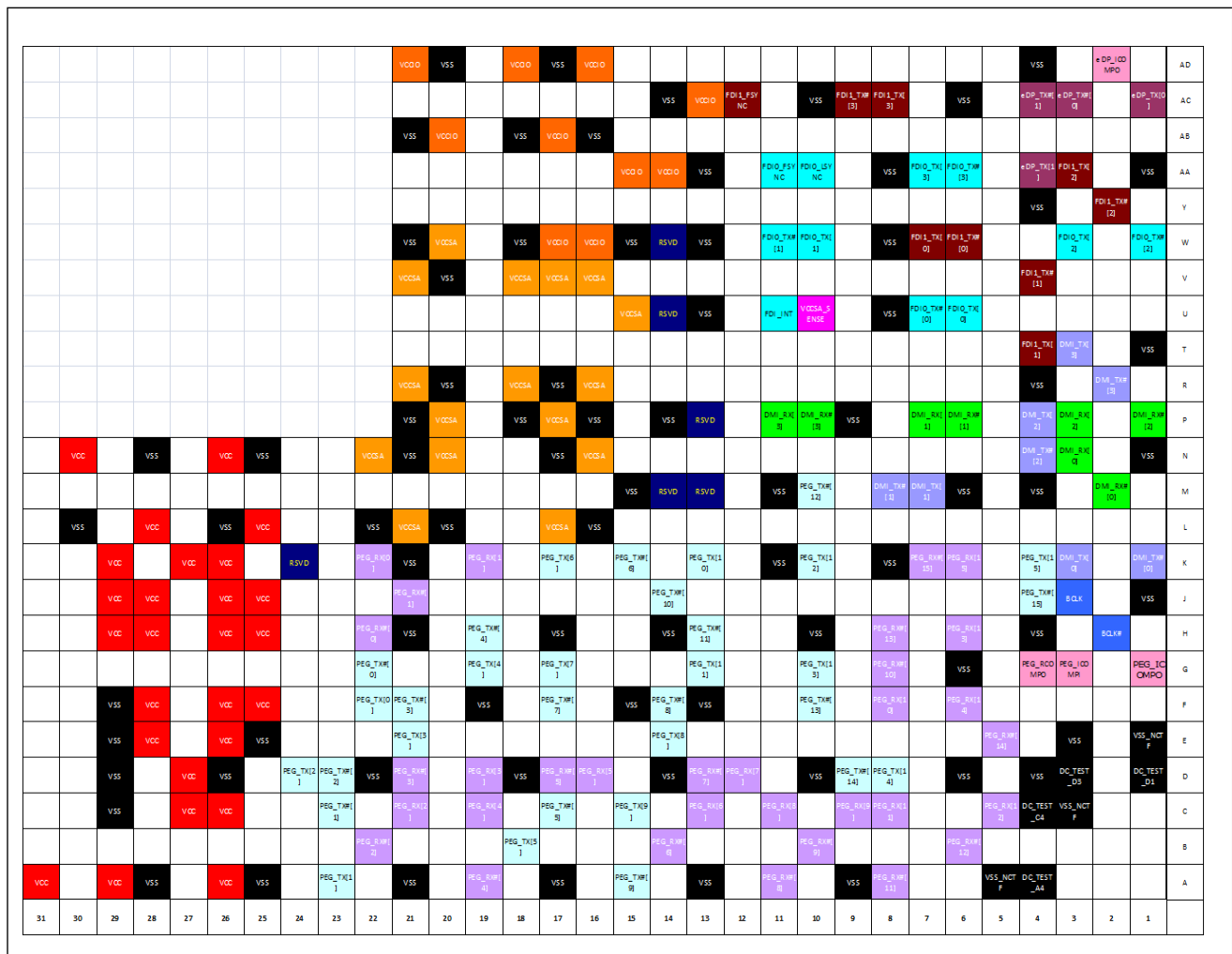
Figure 8-12. BGA1023 Ballmap (Top View, Lower-Right Quadrant)
