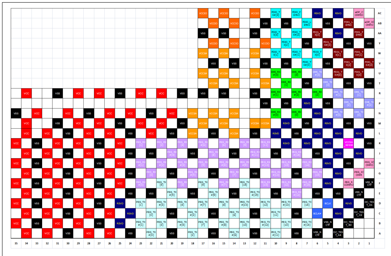
Figure 8-8. BGA1224 Ballmap (Top View, Lower-Right Quadrant)
