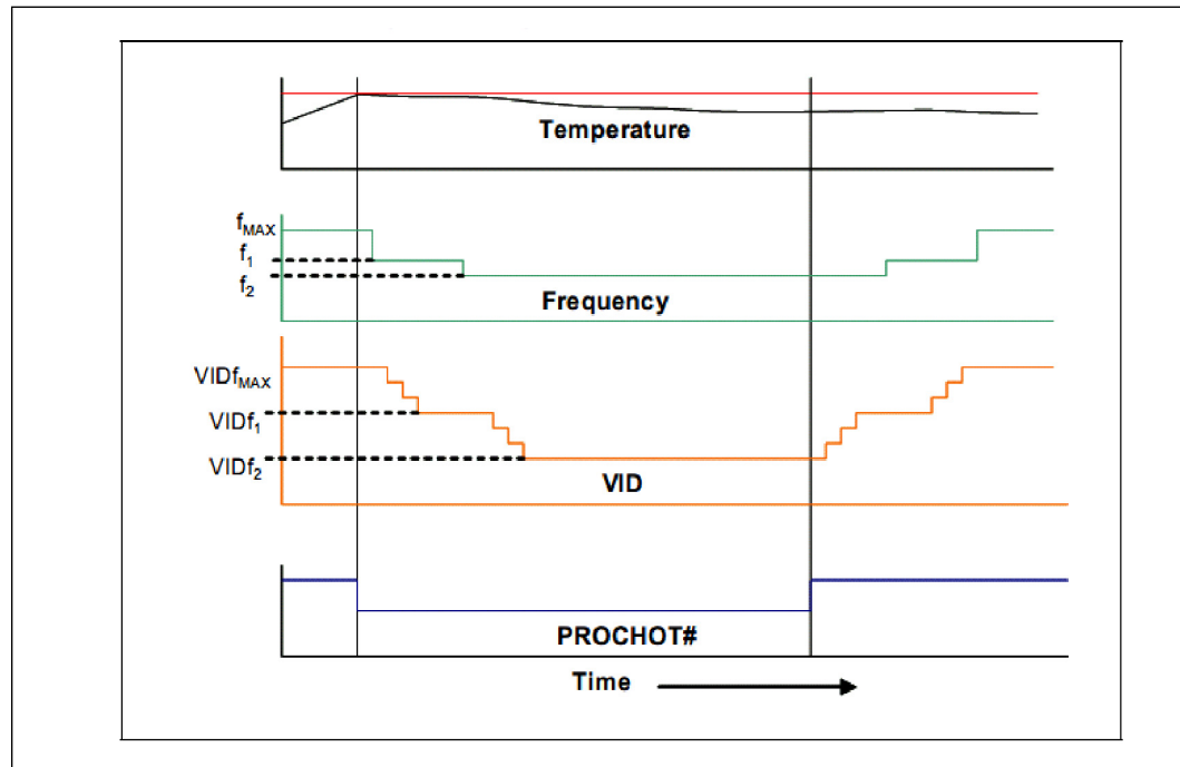
Figure 5-2. Frequency and Voltage Ordering
