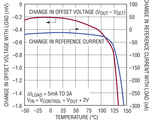
Load Regulation
