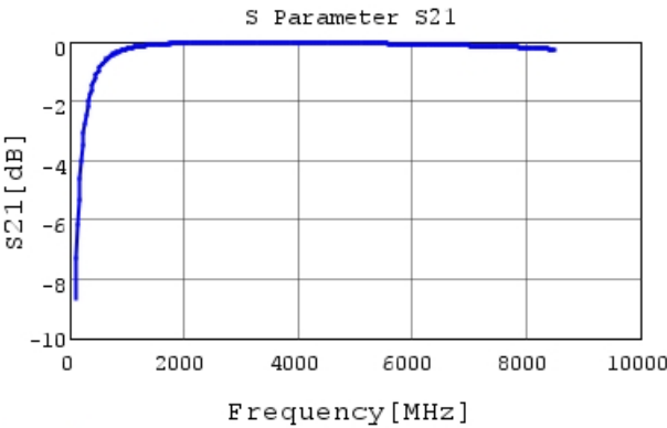
GCQ1555C1H6R3WB01 S21 DCOV, 25degC
