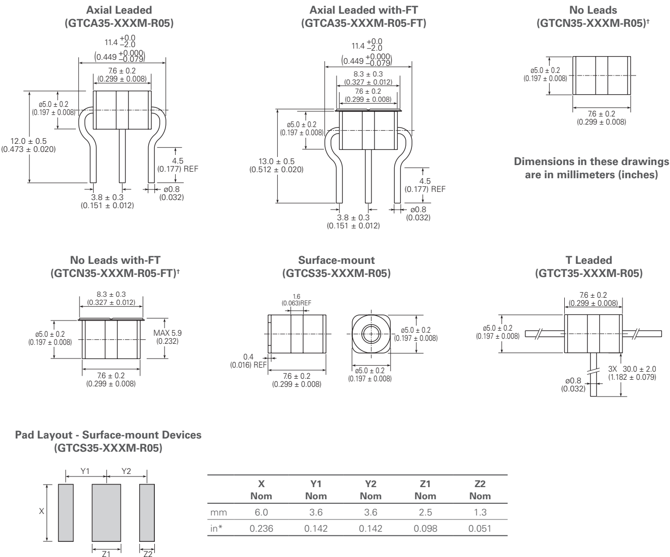
Figure G8 — Three Electrode 5mm Product Dimensions
