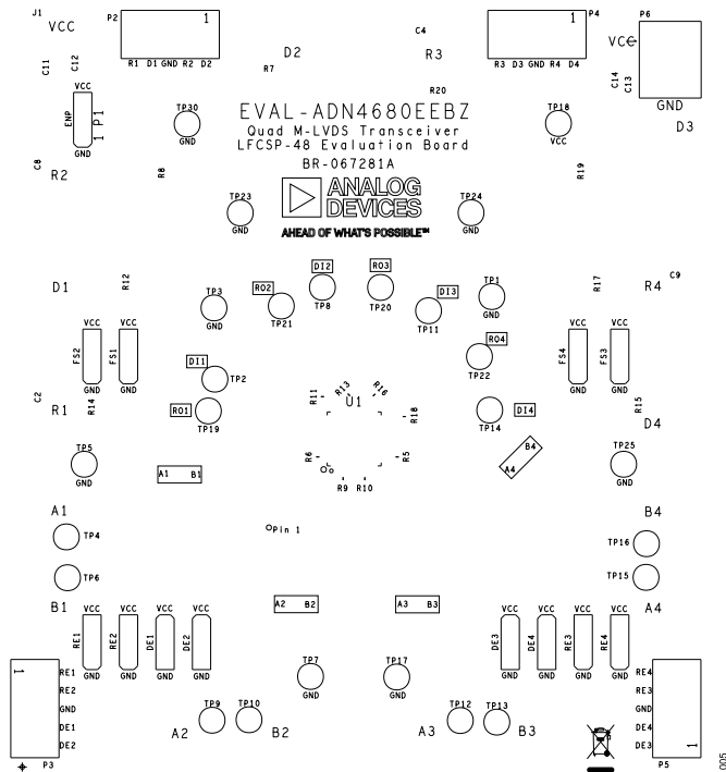
Figure 5. EVAL-ADN4680EEBZ Silkscreen
