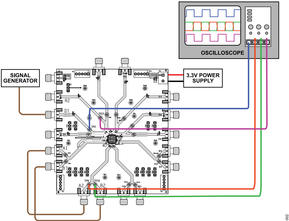
Figure 2. Example Evaluation of the ADN4680E Driver and Receiver
