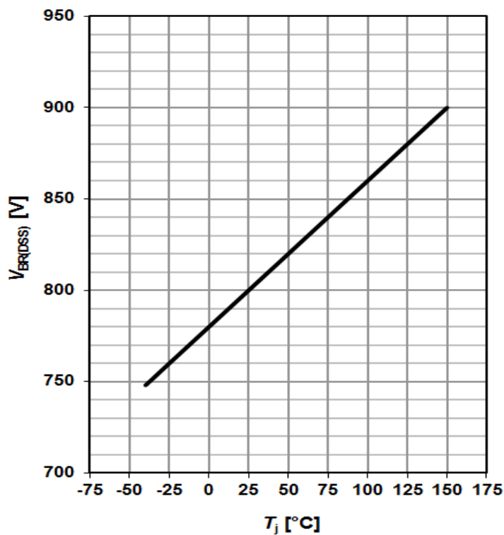
Figure 28 Drain-source breakdown voltage ICE5xRxx80AG; V_{BR(DSS)}=f(T_J) , I_D=1 mA
