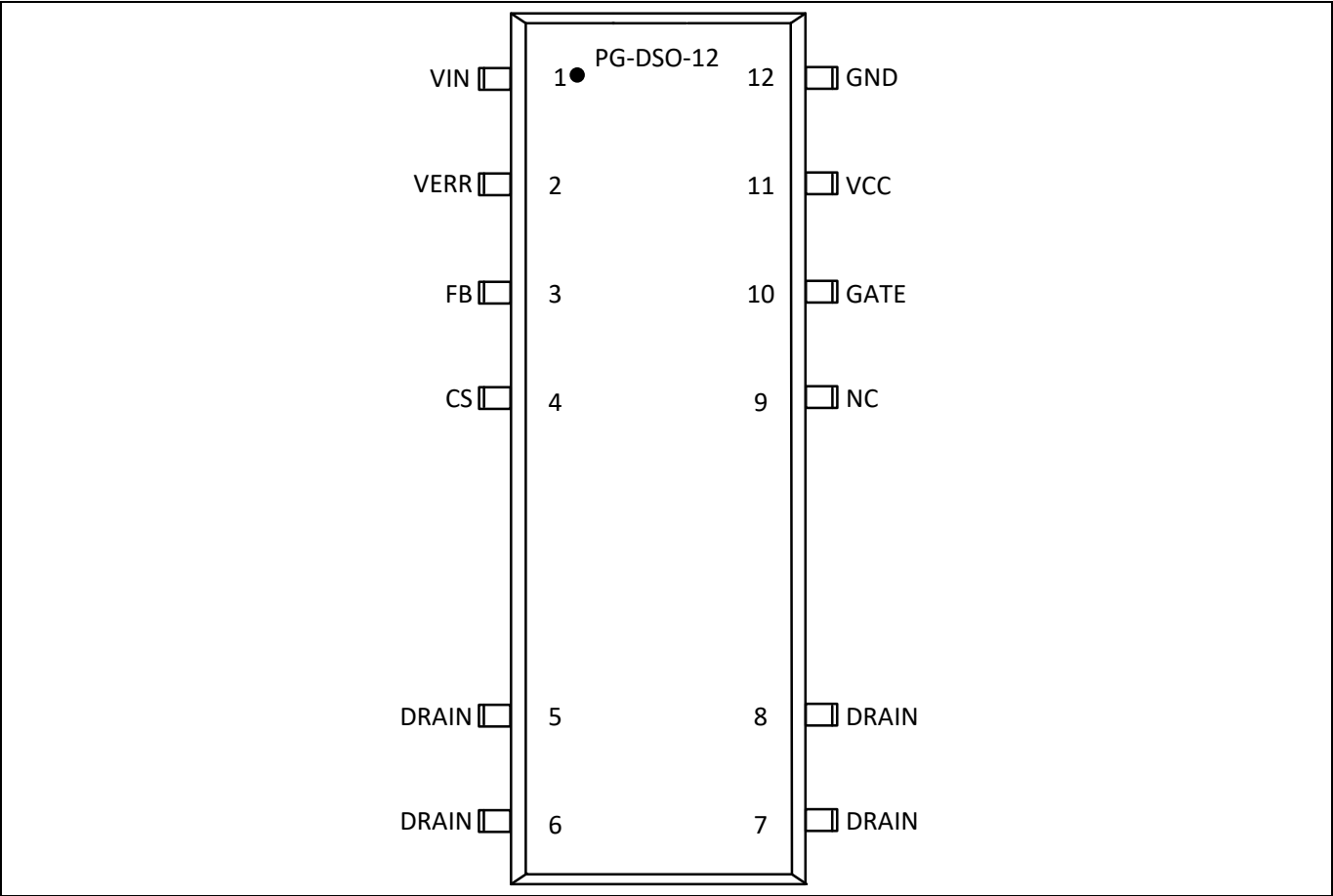
Figure 3 Pin configuration
