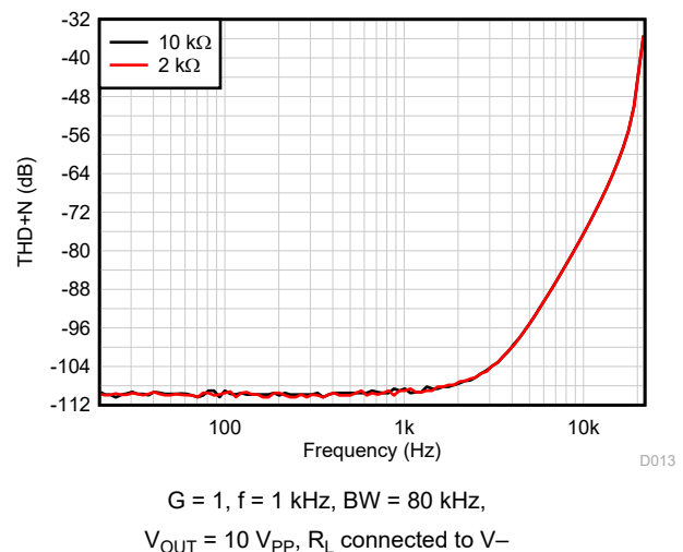
Figure 7-18. THD+N Ratio vs Frequency, G = 1
