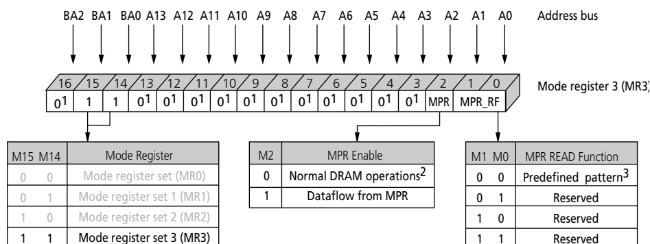
Figure 54: Mode Register 3 (MR3) Definition
