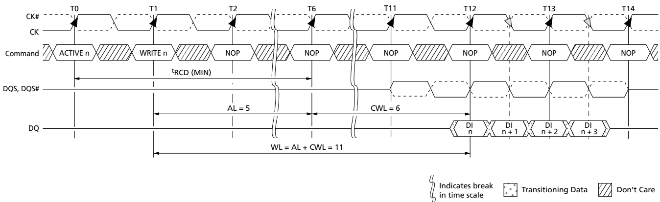
Figure 53: CAS Write Latency
