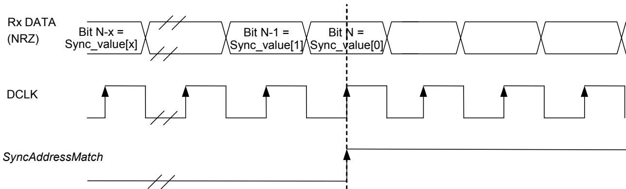
Figure 25. Sync Word Recognition
