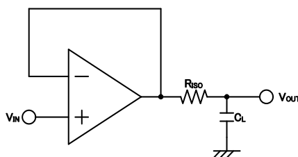
Fig.1. Isolating capacitive load
