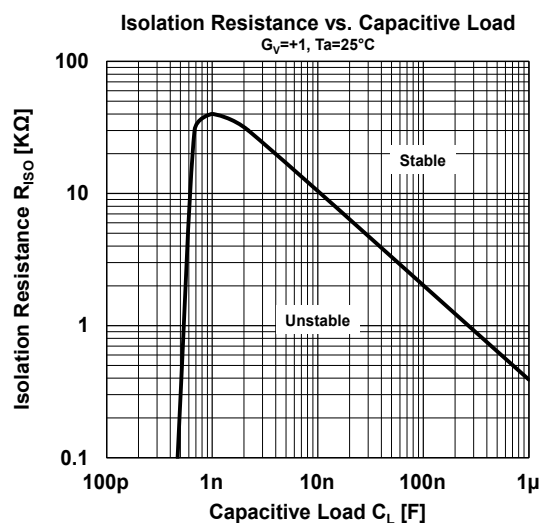
Fig.2. Isolation resistance to improve stability
