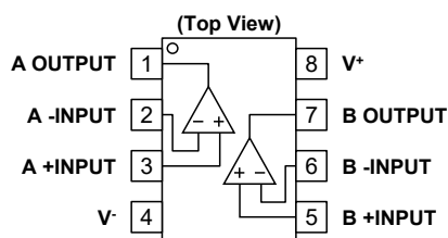
SOP8 (EMP8), MSOP8 (TVSP8)
