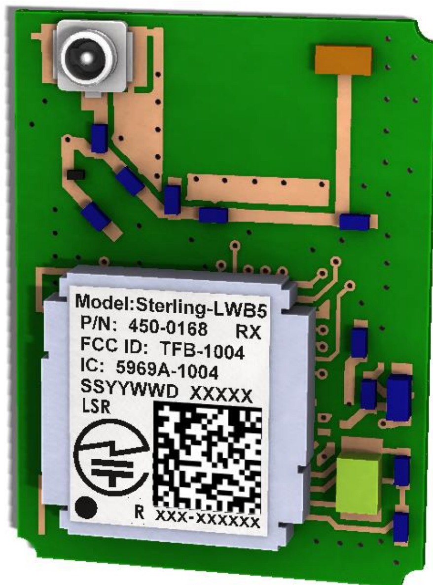
Figure 2 Sterling-LWB5 U.FL Module (450-0168)
