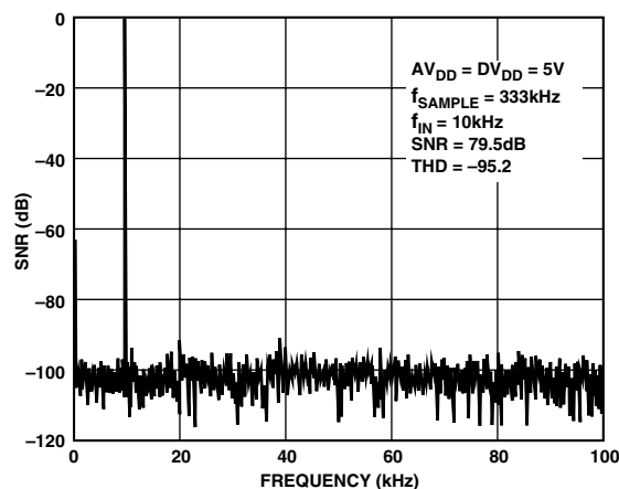
Figure 20. FFT Plot
