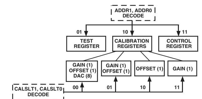
Figure 4. Write Register Hierarchy/Address Decoding
