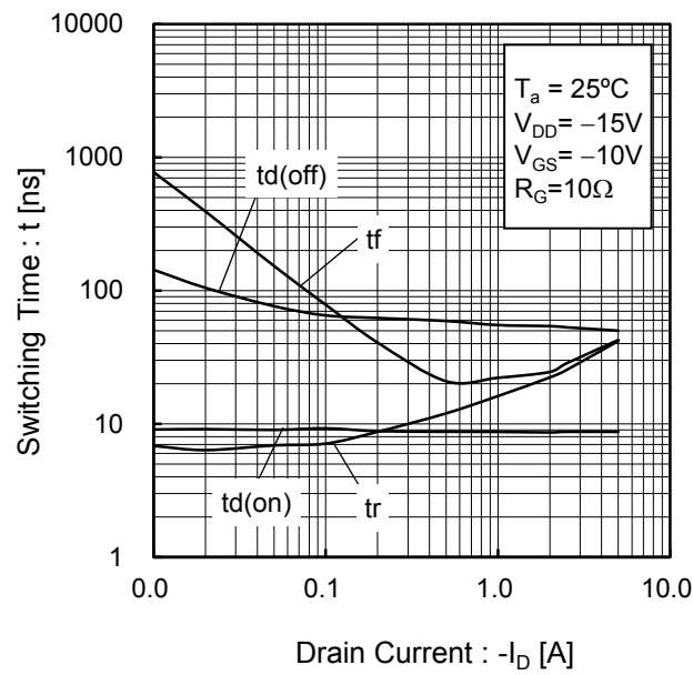
Fig.21 Switching Characteristics
