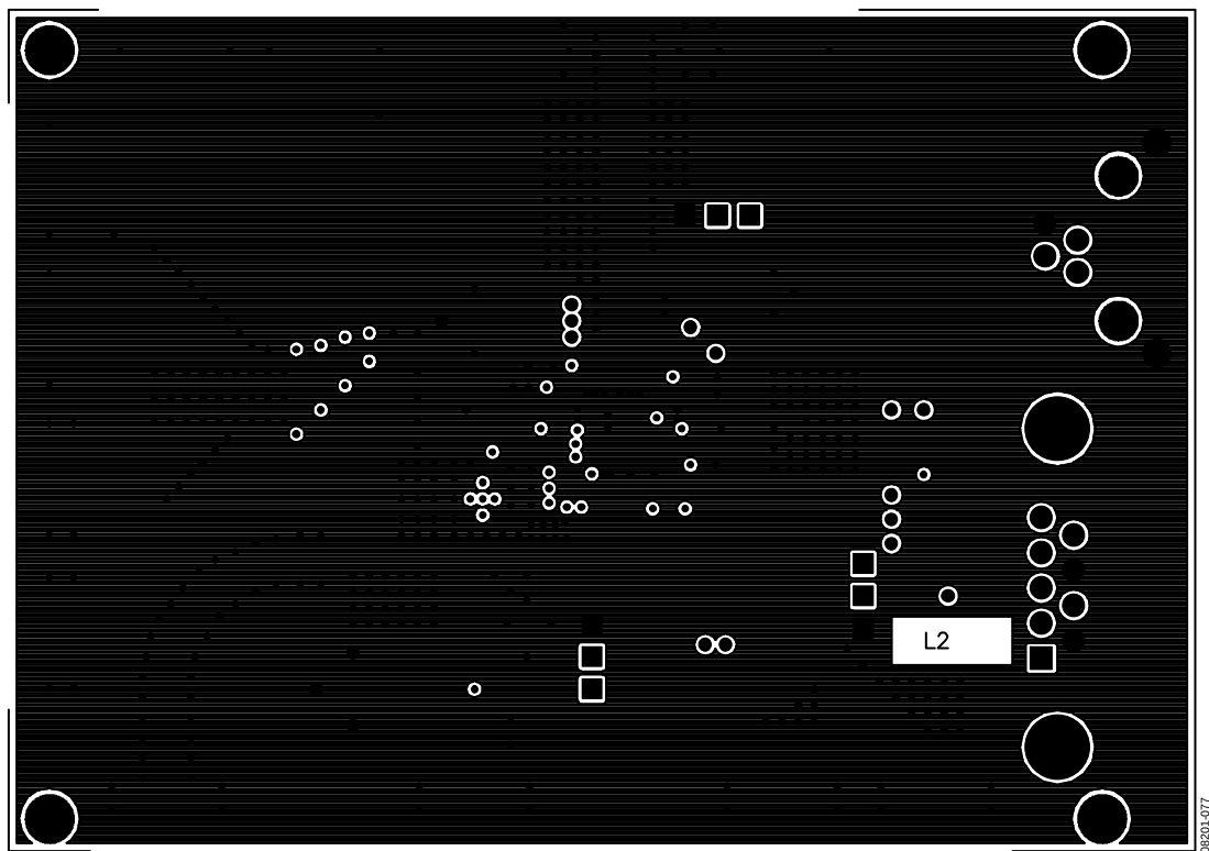
Figure 76. Evaluation Board, Ground—Layer 2
