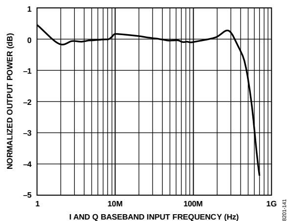
Figure 23. Normalized I and Q Input Bandwidth
