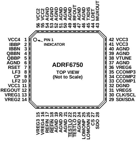
Figure 4. Pin Configuration
