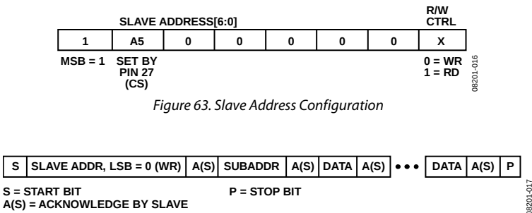
Figure 64. I 2 C Write Data Transfer
