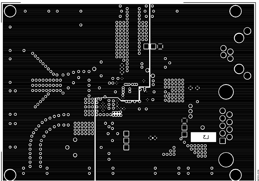
Figure 77. Evaluation Board Power—Layer 3
