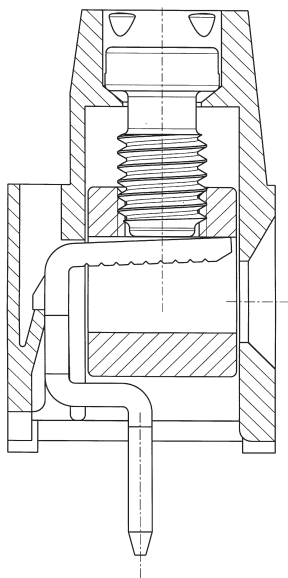
Cross Section One-Piece Connector
