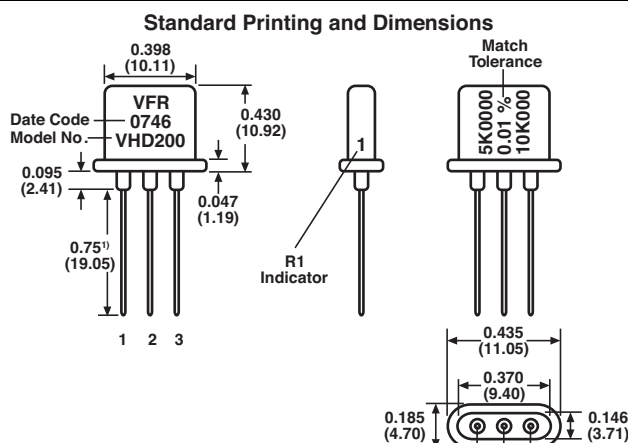
FIGURE 3 - VHD200 AND VHD144 STANDARD PRINTING AND DIMENSIONS in inches (millimeters)
