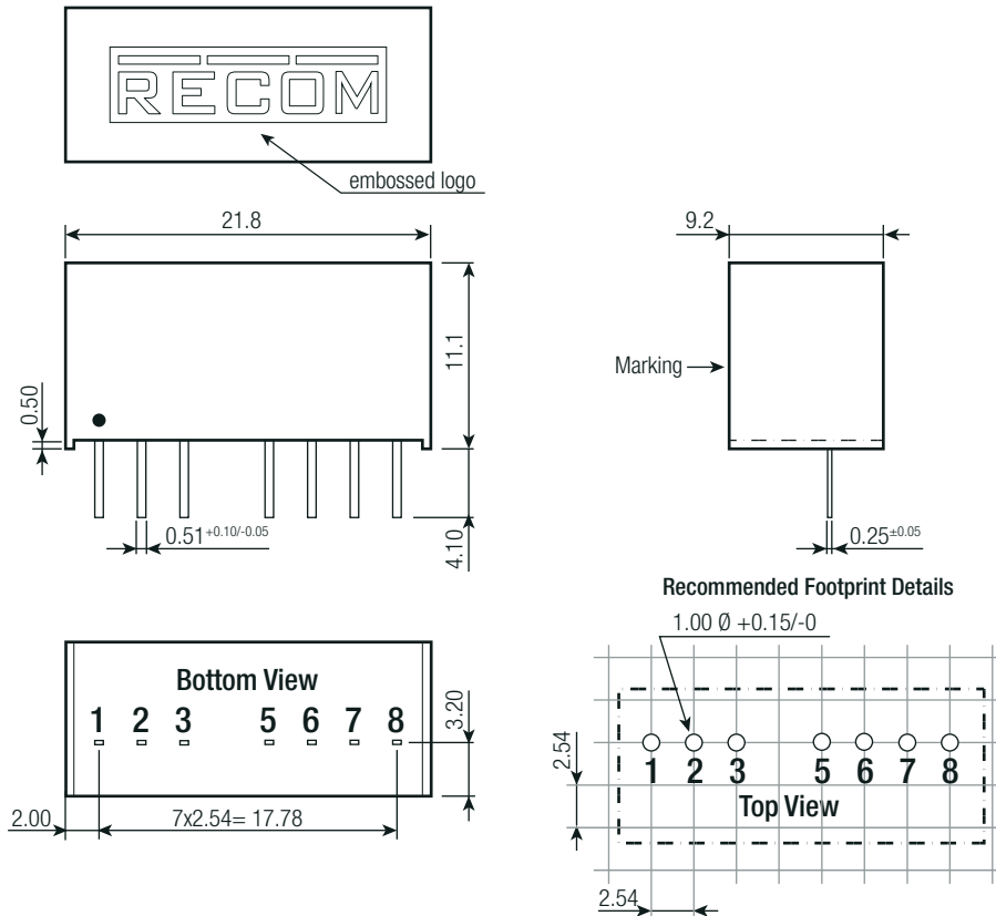
Dimension Drawing (mm)
