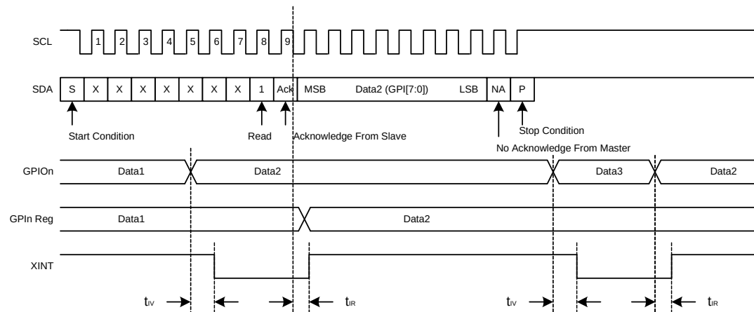
Fig.13 Interrupt Valid/Reset
