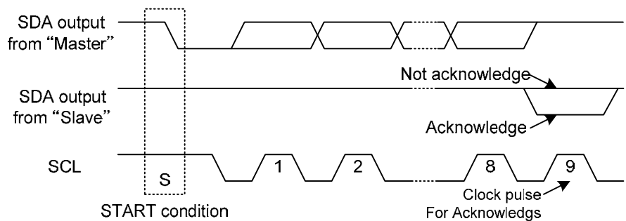
Fig.7 Acknowledge
