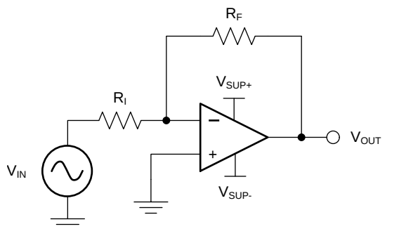
Figure 38. Application Schematic
