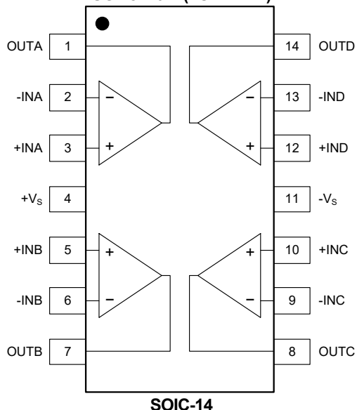
SGM8240-4 (TOP VIEW)
