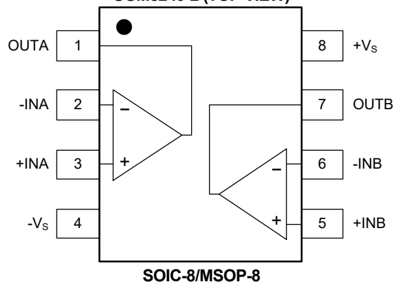
SGM8240-2 (TOP VIEW)
