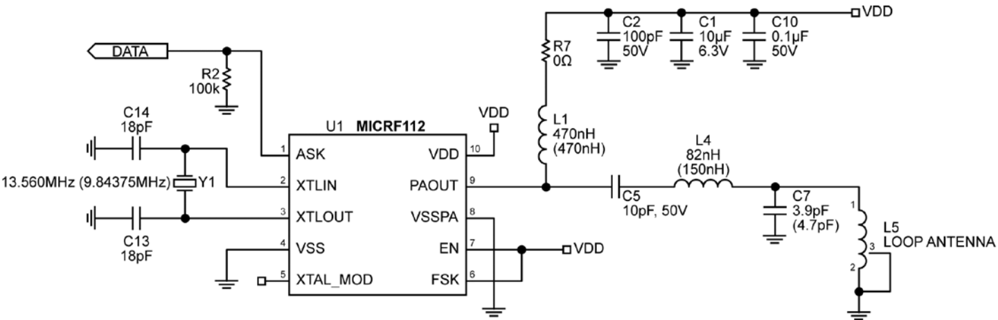
Figure 4. ASK 433.92MHz and 315MHz (MSOP)
