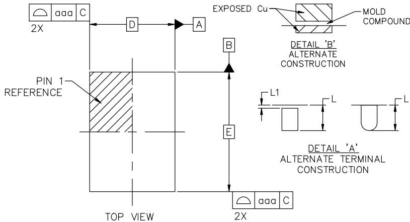
QFN-16, 2.50x3.50x0.90, 0.50P CASE 485AW ISSUE A
