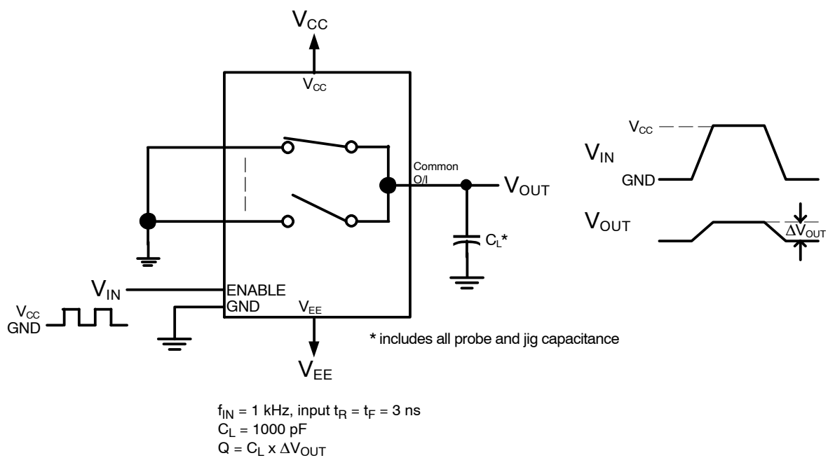
Figure 8. Charge Injection
