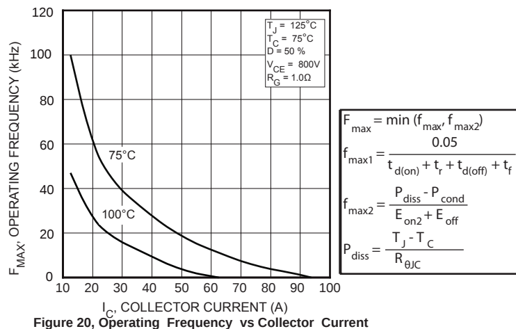
Figure 20, Operating Frequency vs Collector Current
