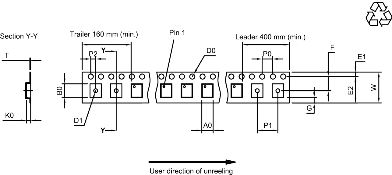
Figure 10: Drawing of tape (first-angle projection) for illustration only and not to scale. The valid tape dimensions are listed in Table 1.
