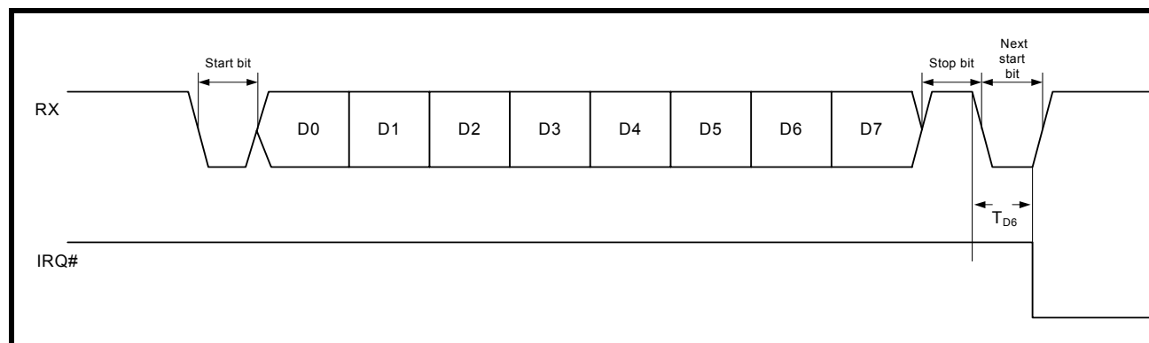
FIGURE 26. RECEIVE INTERRUPT
