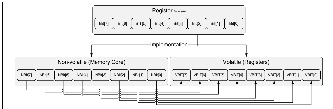
Figure 35 Register structure
