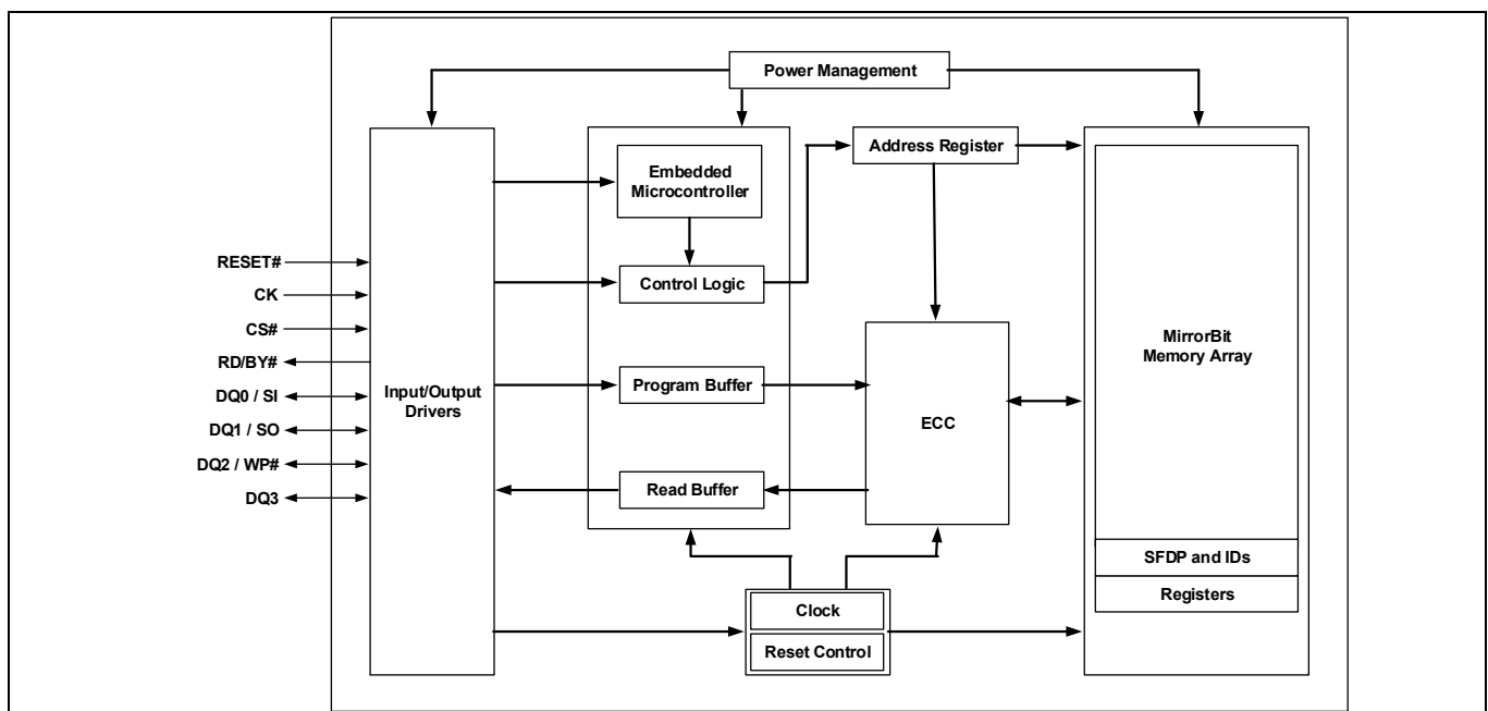
Figure 3 Logic block diagram
