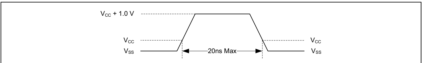
Figure 38 Maximum positive overshoot waveform
