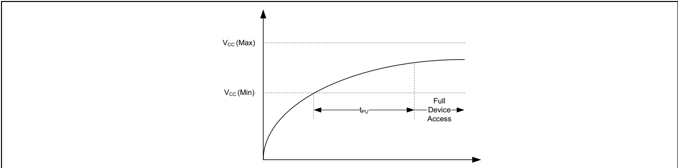
Figure 33 Power up
