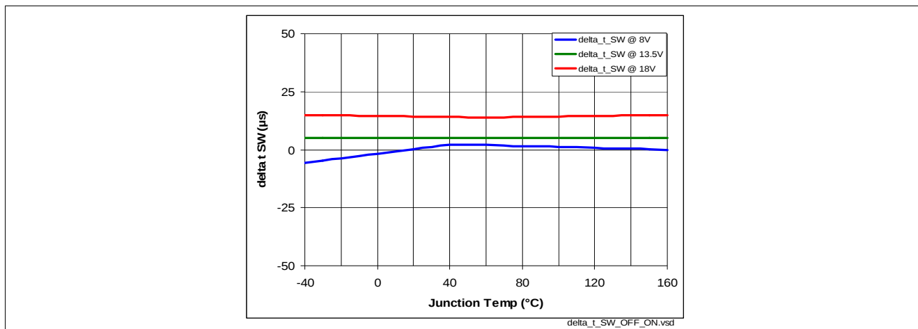
Figure 39 Turn ON / OFF matching \Delta t_{SW} = f(T_J; V_S) , R_L = 4 \Omega
