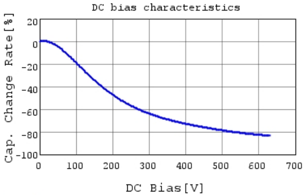
GCJ32DR72J223KXJ1 C-DC bias capchange, 25.0c
