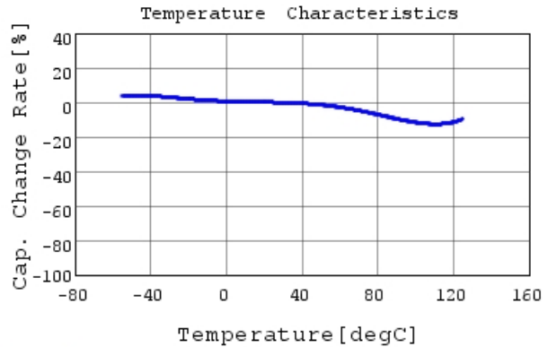
GCJ32DR72J223KXJ1 C-Temp. capchange, DCOV, 1
