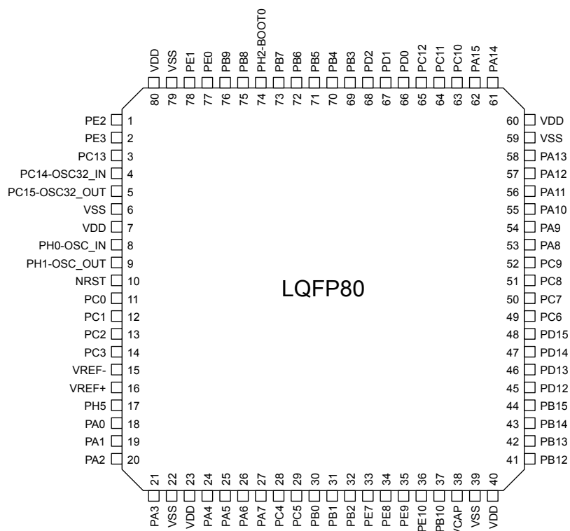
Figure 9. LQFP80 pinout
