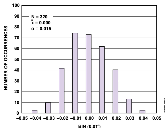
Figure 69. Device to Device Phase Matching, 20 kHz, 25°C, IN3, Normalized to the Mean Value
