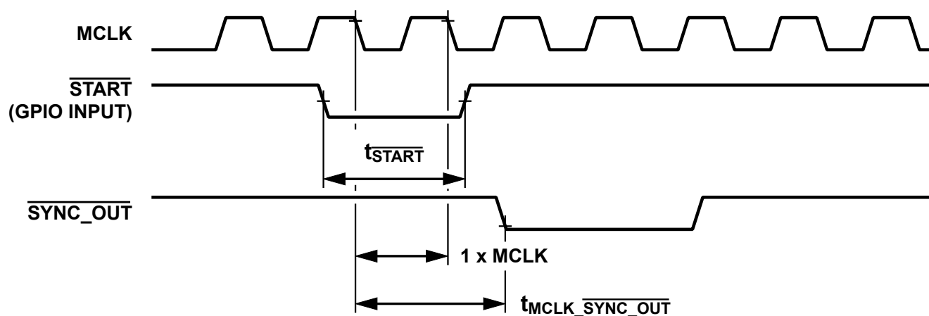
Figure 8. Asynchronous \overline{\text{START}} and \overline{\text{SYNC\_OUT}}
