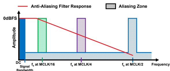
Figure 91. Anti-Alias Filter Response versus MCLK Divider
