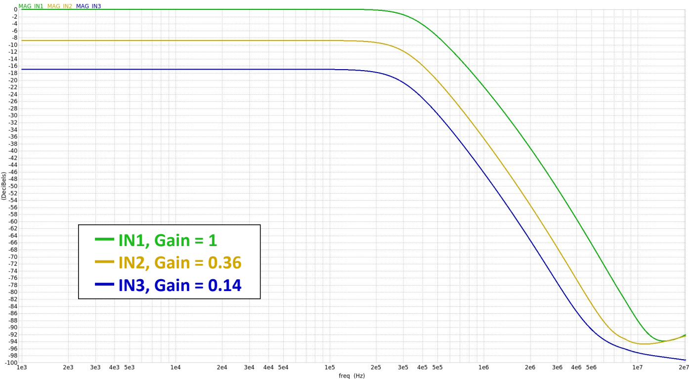
Figure 63. Anti-Aliasing Filter Magnitude Response
