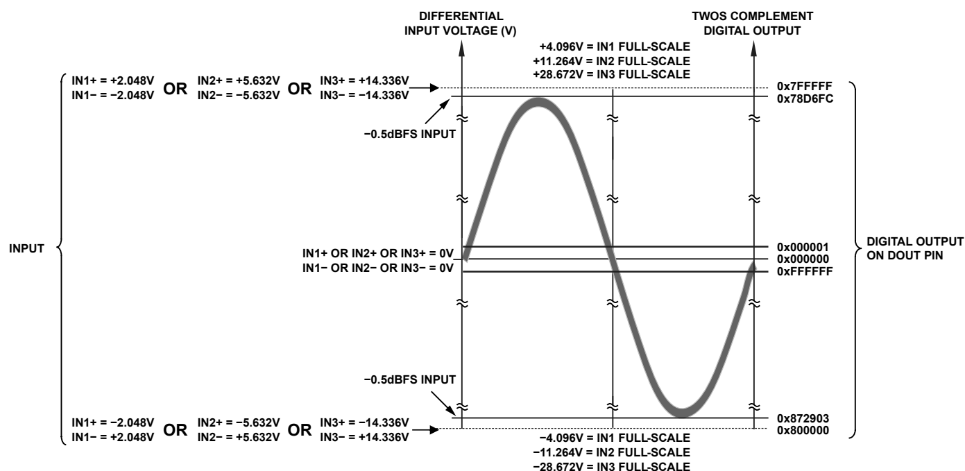
Figure 60. Differential Input Voltage vs. ADC Output Code
