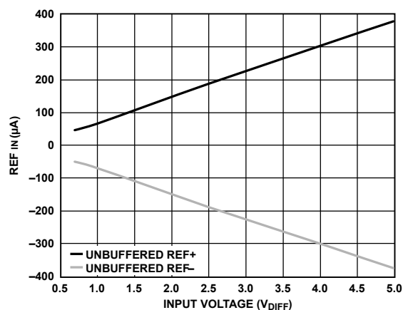
Figure 75. Reference Input Current (REF IN ) vs. Input Voltage, Unbuffered REF+ and REF-
