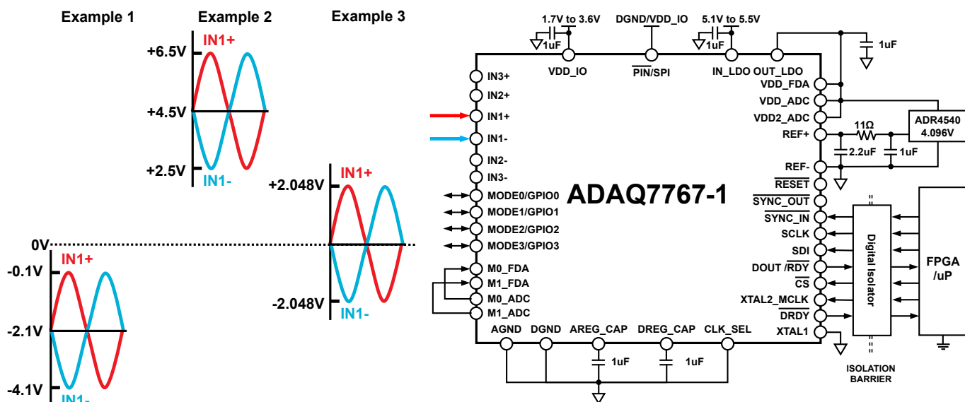
Figure 112. ADAQ7767-1 differential input configuration to IN1+/- ( AFE\_GAIN = 1 V/V )
