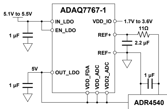
Figure 78. ADAQ7767-1 Power Supply Connection Using Internal LDO
