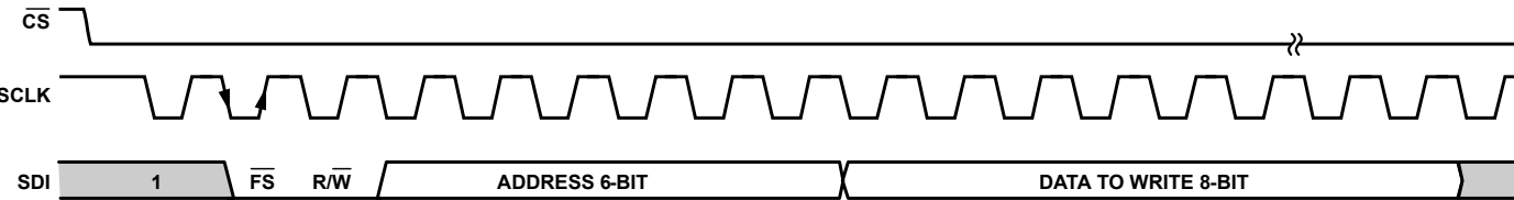
Figure 99. 3-Wire SPI Write Frame ( \overline{CS} = 0 )
