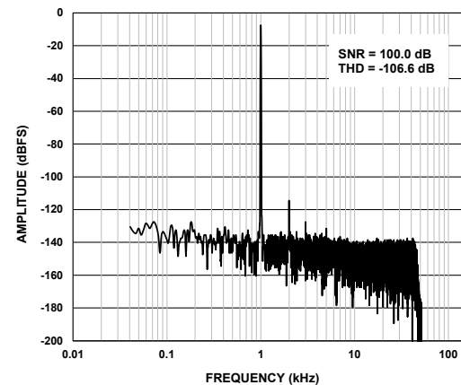
Figure 17. Wideband Low Ripple FIR Filter, MCLK = 13.107 MHz, ODR = 102.4 kSPS, Single-Ended Input, IN3, -12 VDC + 10 Vp [-2V to -22V]
