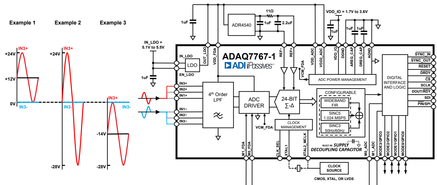
Figure 1. Block Diagram
