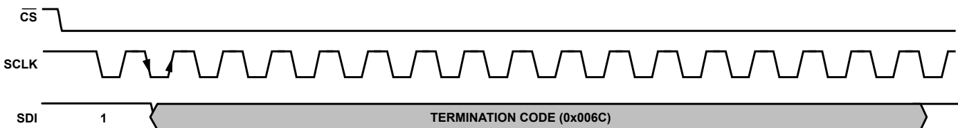
Figure 106. Exiting Continuous Read Mode ( \overline{CS}=0 )
