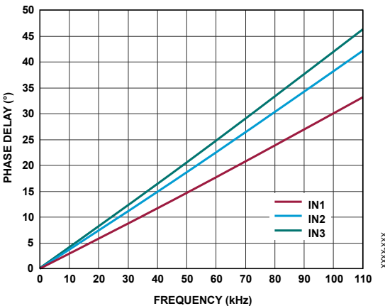
Figure 42. Analog Front-End (AFE) Passband Phase Response
