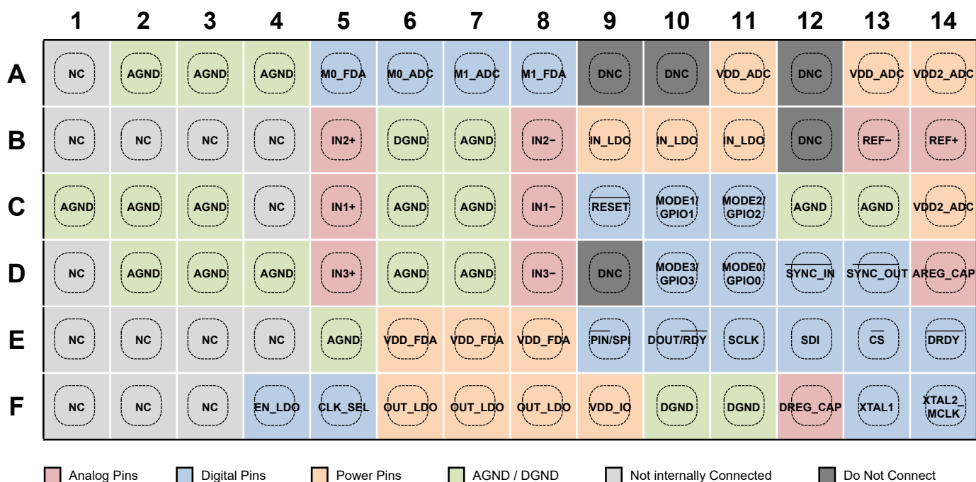
Figure 13. Pin Configuration
