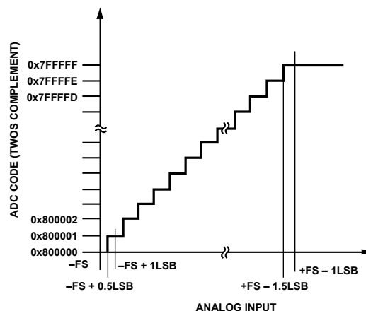
Figure 77. Ideal Transfer Function (FS is Full-Scale)
