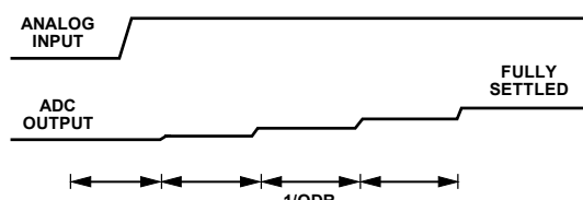
Figure 88. Sinc5 Filter Step Response
