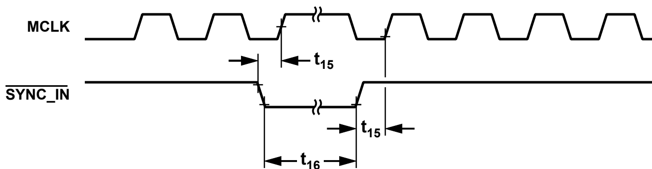
Figure 7. Synchronous \overline{\text{SYNC\_IN}} Pulse
