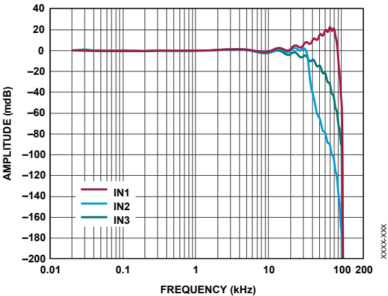
Figure 40. Wideband Low Ripple FIR Filter Magnitude Flatness, ODR = 256 kSPS
