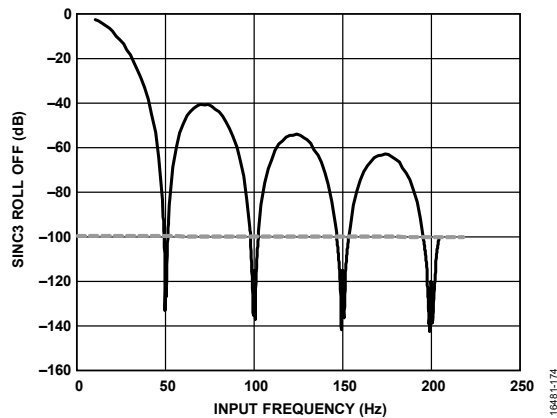
Figure 89. Sinc3 Filter Frequency Response Showing 50 Hz Rejection, 50 Hz ODR, \times 163,840 Decimation
