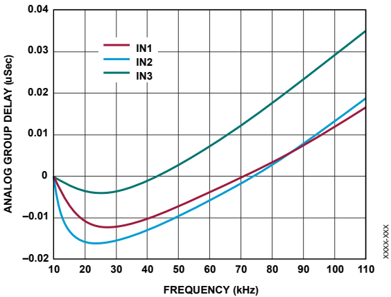
Figure 41. Analog Front-End (AFE) Passband Analog Group Delay vs. Frequency at 25°C, Normalized to Delay at 10 kHz
