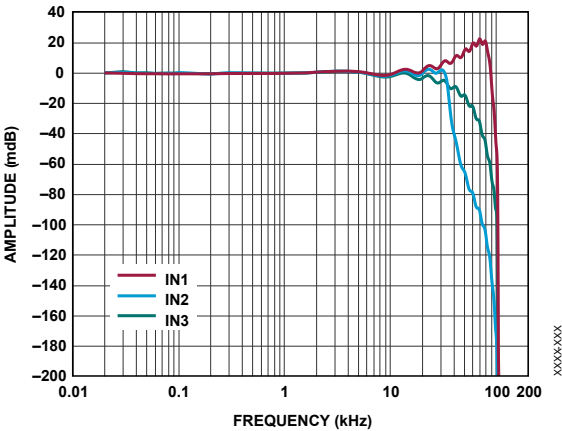
Figure 65. AAF Passband Droop for Various Input Ranges
