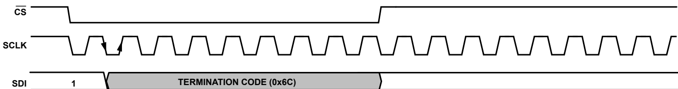
Figure 105. Exiting Continuous Read Mode ( \overline{CS} Toggling)
