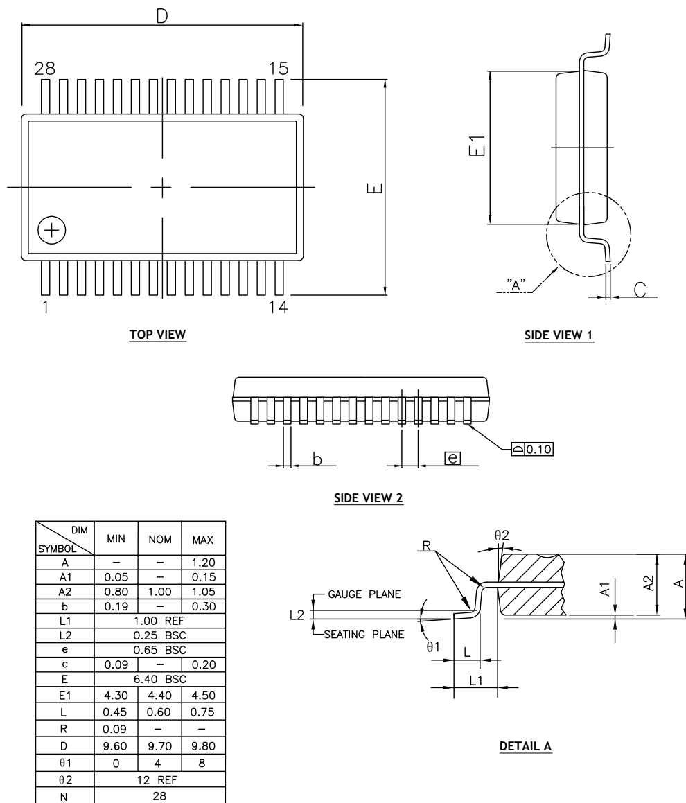
TERMINAL DETAILS
