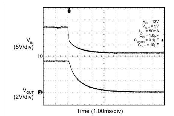
FIGURE 2-20: Fast Turn-Off.
