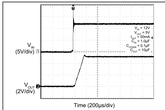
FIGURE 2-19: Fast Turn-On.
