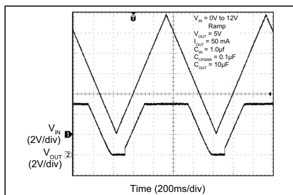
FIGURE 2-21: V_{IN} UVLO Threshold.
