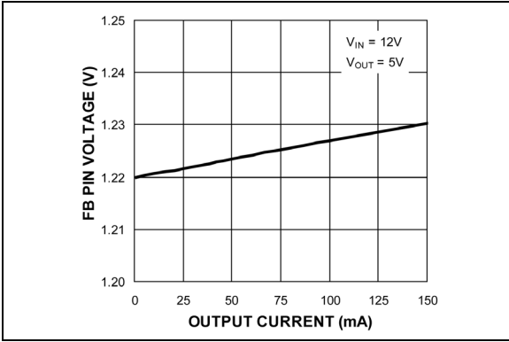
FIGURE 2-11: Feedback Pin Voltage vs. Output Current.
