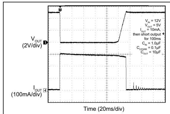
FIGURE 2-22: Current Limit.
