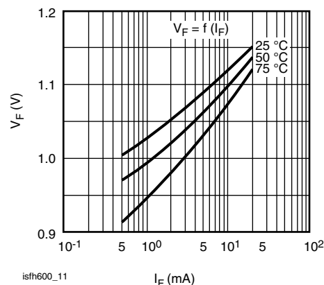
Fig. 11 - Forward Voltage
