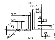
● Mounting drawing
