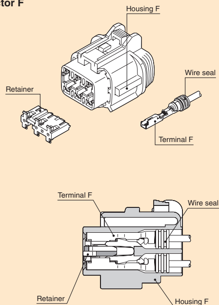
Connector F
