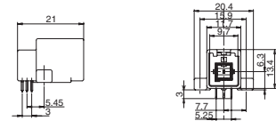
● Dimensional drawing
