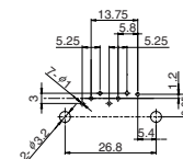
● Mounting drawing
