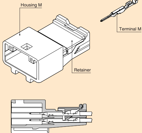
Connector M
