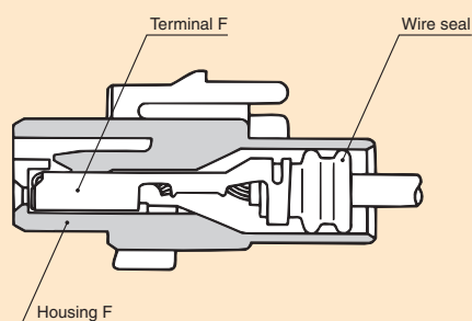
Connector F
