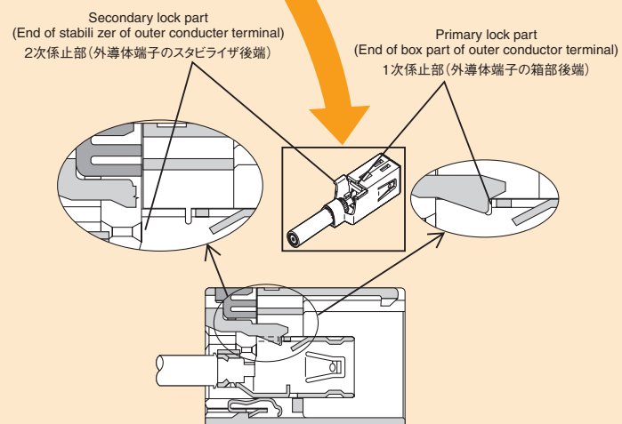
Secondary lock structure of HFC HFCの2重係止構造
