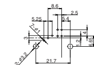
● Mounting drawing
