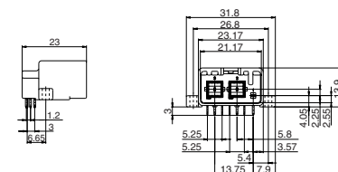
● Dimensional drawing
