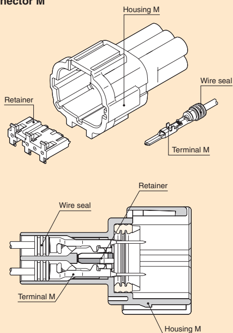
Connector M
