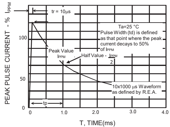
FIG.2 - PULSE WAVEFORM
