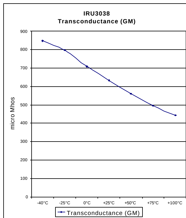
Figure 9 - Transconductance of IRU3038.
