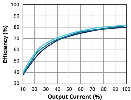
EFFICIENCY VS OUTPUT LOAD PCN1-S12-S5-M
