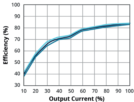
EFFICIENCY VS OUTPUT LOAD PCN1-S12-S12-M
