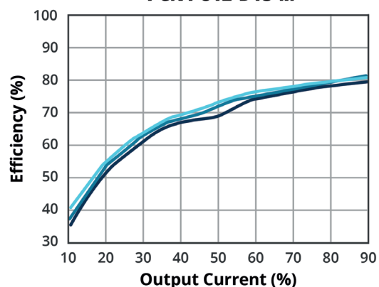
EFFICIENCY VS OUTPUT LOAD PCN1-S12-D15-M
