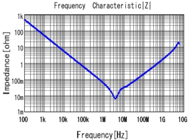
■ GRM219C81A475KE34 |Z| DC0V, 25degC
