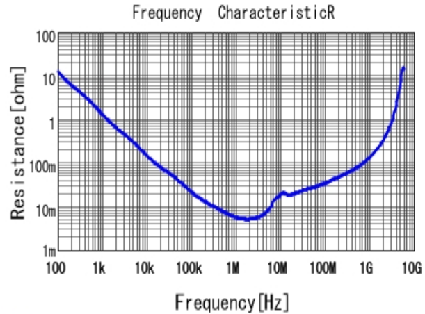
■ GRM219C81A475KE34 R DC0V, 25degC
