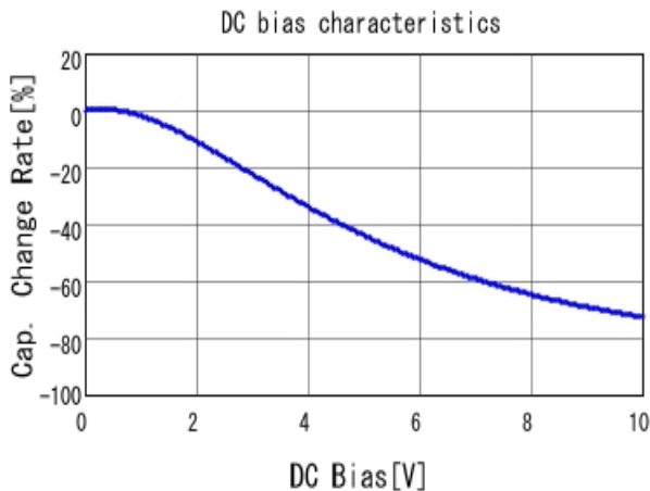
■ GRM219C81A475KE34 C-DC bias capchange, 25.0degC, AC0.
