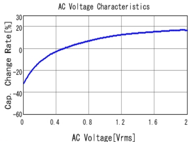
■ GRM219C81A475KE34 C-AC Voltage capchange, DC0V, 25.0d
