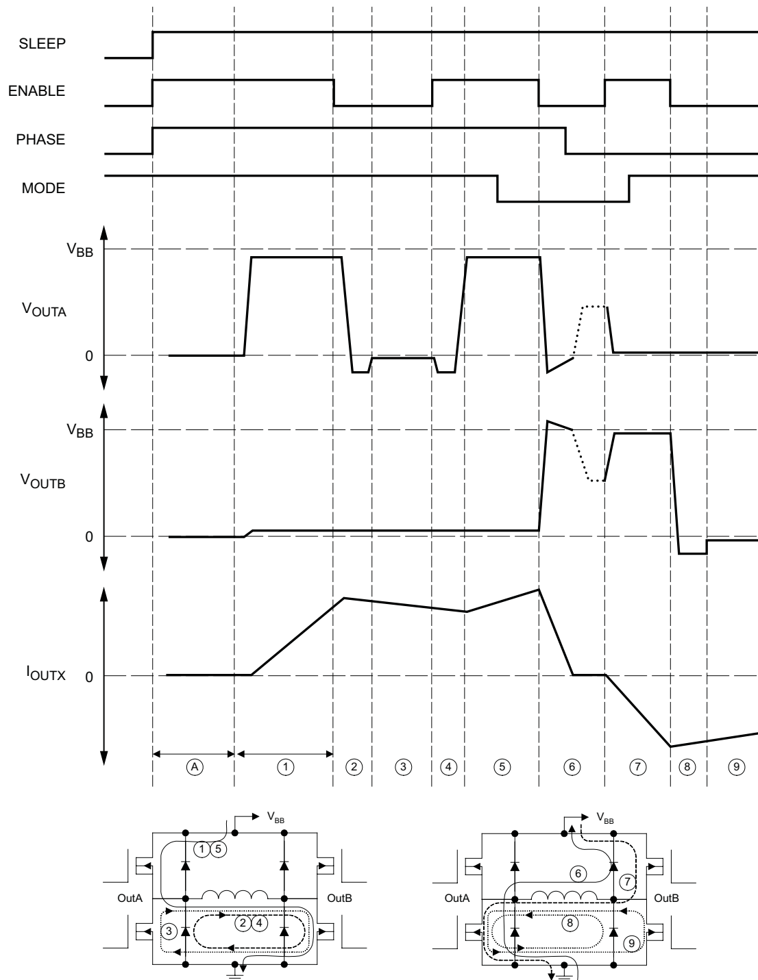
Timing Diagram: PWM Control
