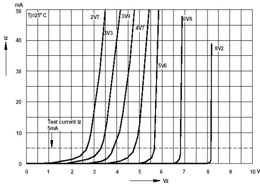
Figure 1. Breakdown Characteristics @ T J =Constant (pulsed)
