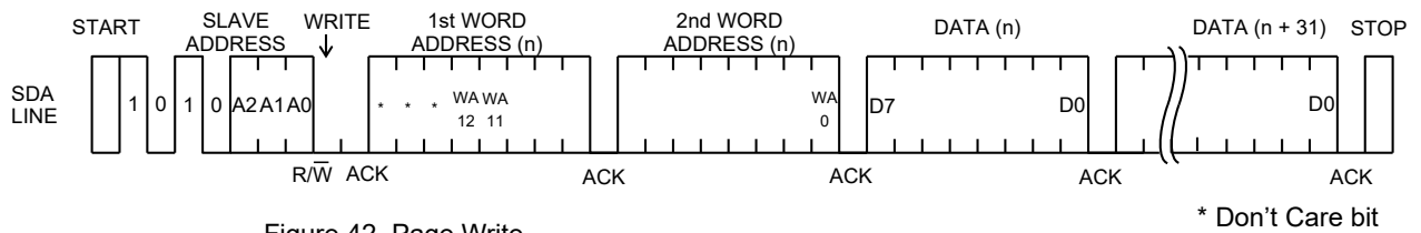
Figure 42. Page Write
