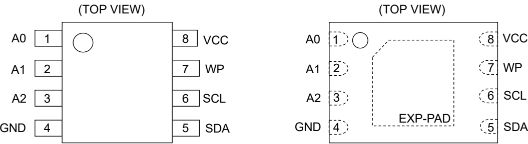
Figure 3-(a). Pin Configuration (SOP8 *1 , SOP-J8, TSSOP-B8, MSOP8) *1 Last Time Buy. Figure 3-(b). Pin Configuration (VSON008X2030 *1 , VSON08AX2030) *1 Last Time Buy.
