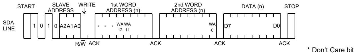
Figure 41. Byte Write
