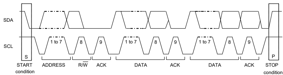
Figure 40. Data Transfer Timing
