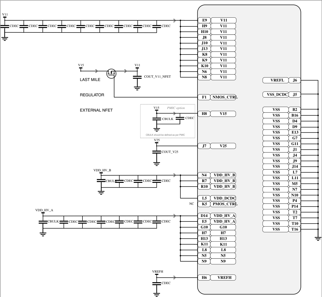
Figure 28. 289BGA package decoupling capacitor pinout diagram, (S32K388)
