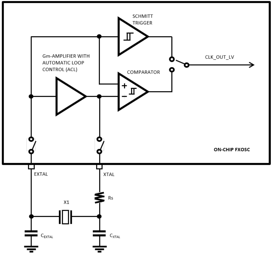
Figure 45. Block diagram
